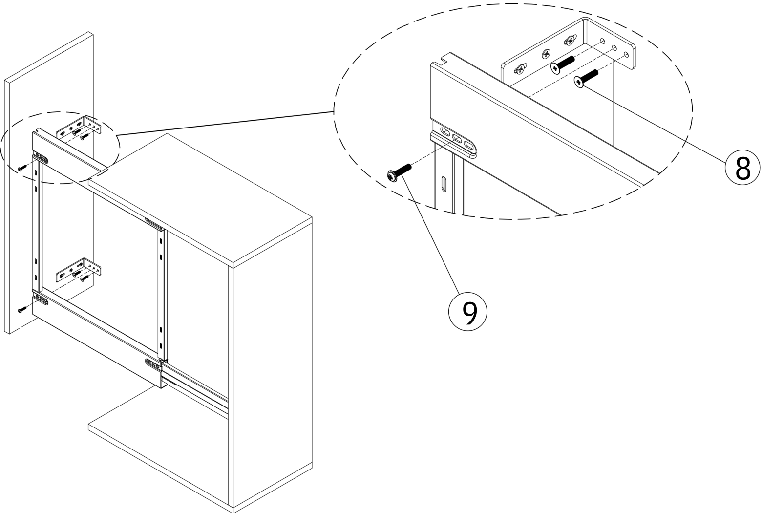
3.3 Door panel installation
